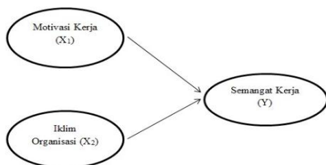
Gambar 1 Model Penelitian
